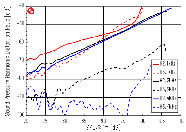
Figure 11 Sound Pressure Harmonic Distortion, 0-14Vrms
