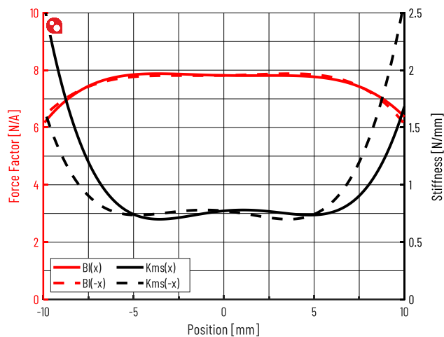
Figure 3 Force Factor and Stiffness vs Voice Coil Position
