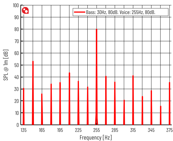
Figure 10 Intermodulation Distortion @ 30Hz 80dB, 255Hz 80dB
