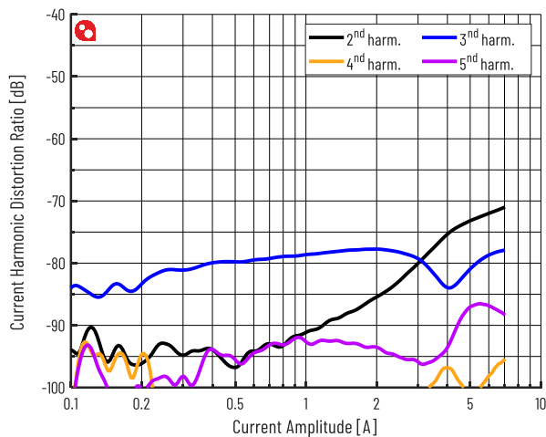
Figure 8 Current Harmonic Distortion @ 1kHz, 0-28.3Vrms
