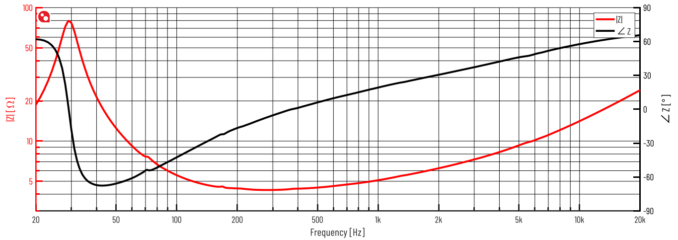
Figure 2 Impedance Response @ 2.83V
