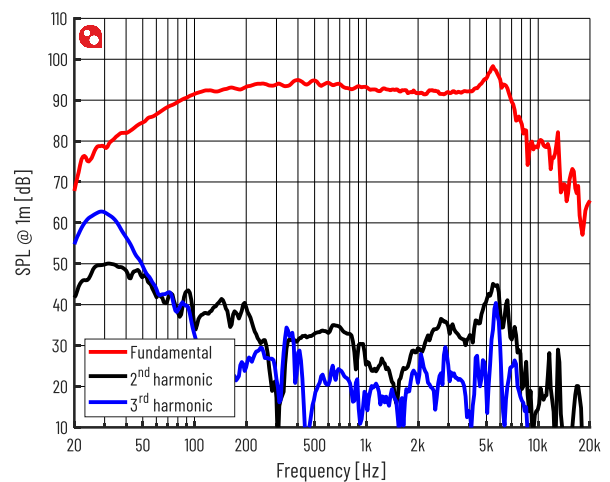
Figure 6 Frequency Response @ 1m, 94dB
