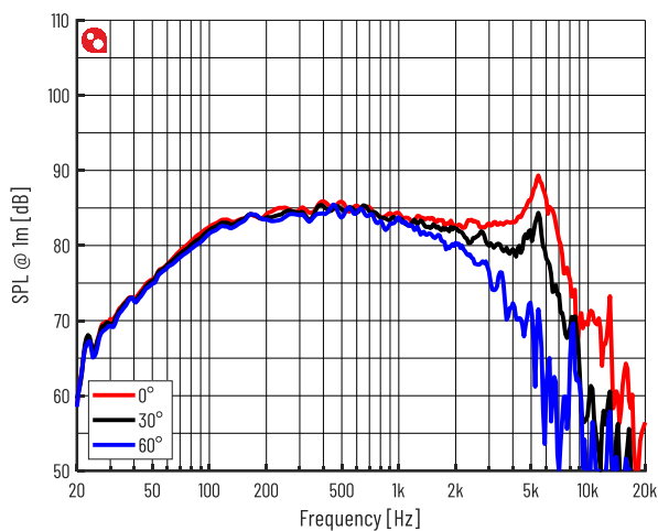
Figure 5 Axial Frequency Response @ 1m, 2.83Vrms
