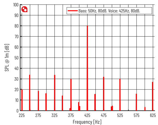
Figure 11 Intermodulation Distortion @ 50Hz 80dB, 425Hz 80dB
