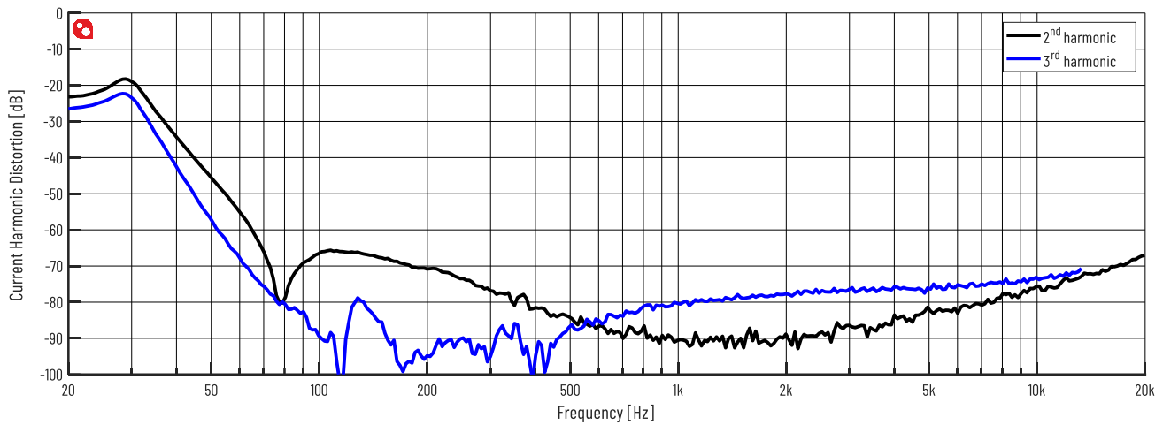
Figure 7 Current Harmonic Distortion @ 2.83Vrms
