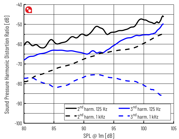
Figure 9 Sound Pressure Harmonic Distortion @ 1m, 0-28.3Vrms
